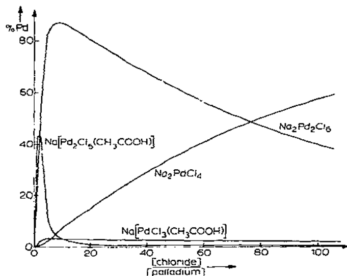
Fig. 3. Percentage of palladium(II) present in each form as a function of the ratio of the concentrations of chloride and palladium(II).
